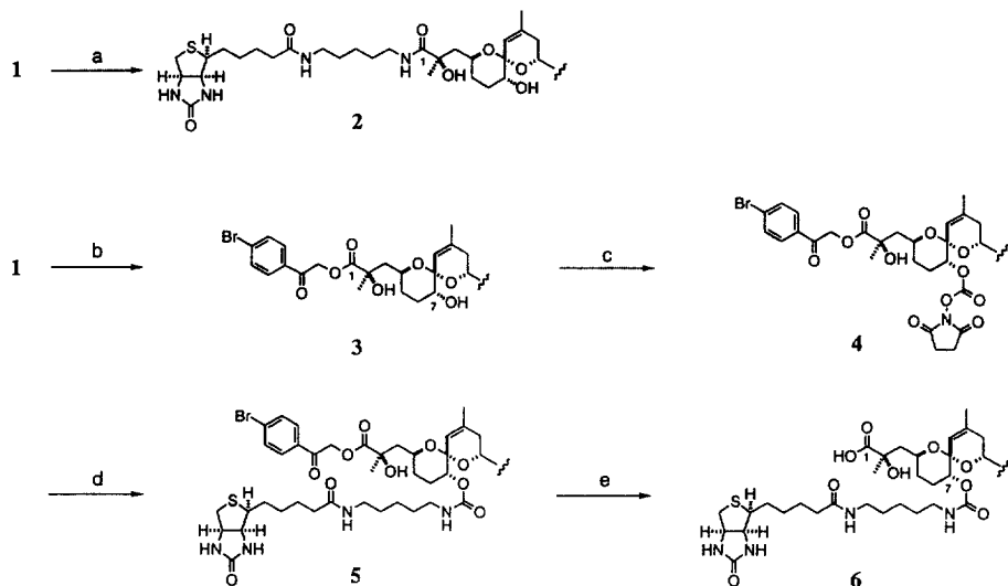
Scheme. (a) 5-(biotinamido)pentylamine, HOBt, EDC·HCl, Et 3 N, DMF, rt, 4h, 40%; (b) p -bromophenacyl bromide, Et 3 N, acetone, 40°C, 3h, 93%; (c) N,N' -disuccinimidyl carbonate, Et 3 N, CH 3 CN, rt, 5h; (d) 5-(biotinamido)pentylamine, Et 3 N, DMF, rt, 12h; (e) Zn, AcOH, rt, 5h, 54% in 3 steps.
