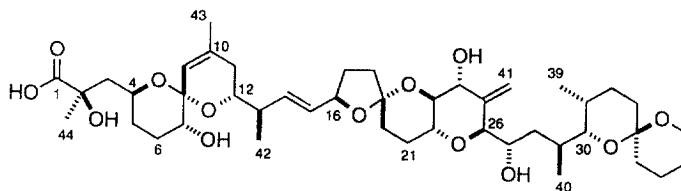
Okadaic acid (1)
