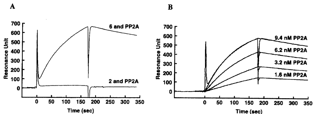
Fig. 1. Sensorgrams of the interactions between the biotin-conjugates of okadaic acid and PP2A. (A) Interactions of 2 and 6 with 9.4 nM PP2A. (B) Dependence of the binding of 6 on the concentration of PP2A.
